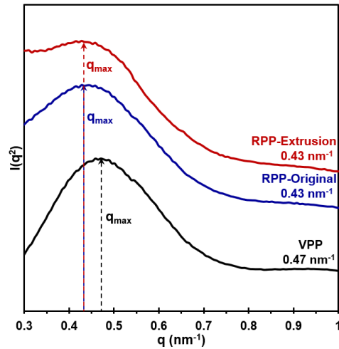
Figure 1 SAXS profile of VPP, RPP-Original, and RPP-Extrusion.
