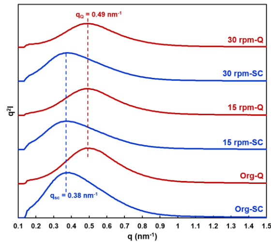
Fig. 2 SAXS profile of LDPE original samples (Org) and LDPE after mixing treatment with different mixing rate (15 or 30 rpm) and remolding condition (SC; showed in blue color curve, or Q; showed in red color curve).
