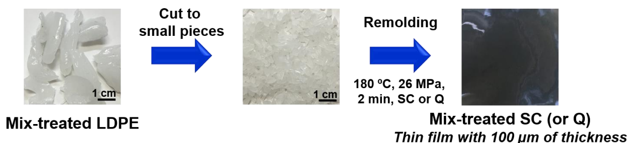
Fig. 1 Fabrication of thin film (100 μm of thickness) by hot compression
